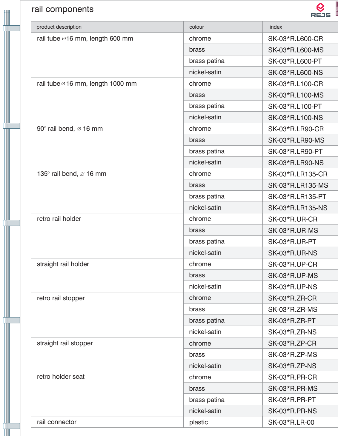
90° rail bend
