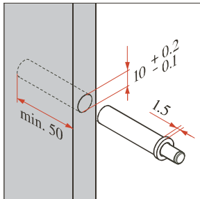
BLUMOTION for doors carcass plate mounting method
