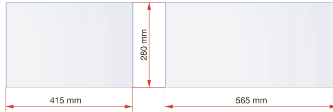
upper inserted glass shelf "45"
