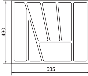
METABOX 60
