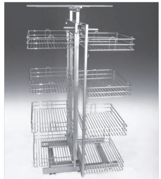
Magic MIDI basket for application in corner cabinets DNWL(P)-105/136-L (-P), DNWL(P)-105/143-L (-P) attached: to bottom of upper crown of carcass; dimensions: 670 / 500 / 1100-1500 mm (width/depth/height)
