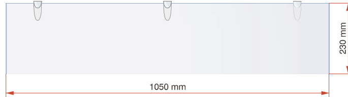
glass shelf "105"
