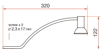
halogen 12V mounting, bulb type G5, 3-35W
