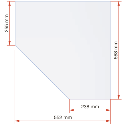
corner inserted glass shelf
