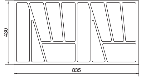
METABOX 90
