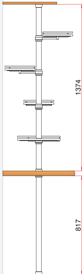
KU003 storage column
