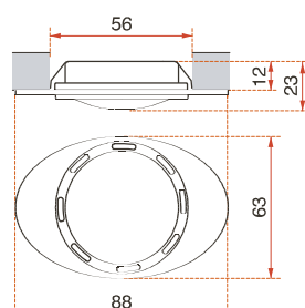
halogen 12V mounting pressed, bulb type G4-20W
