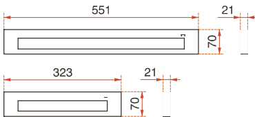
mounting SELENE 8W
