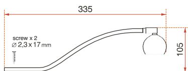
halogen 12V mounting with movable head, bulb type G5, 3-35W
