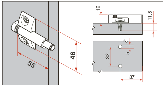
EXPANDO cross plate mounting method
