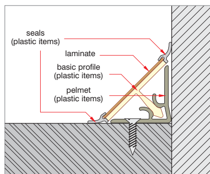
method of mounting splash-back batten in worktop colours, type II
