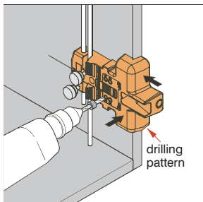
Drilling carcass under mounting plate (both types)
