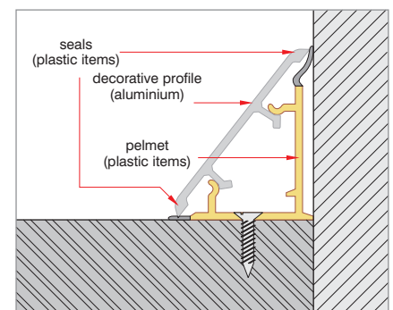
method of mounting aluminium splash-back batten
