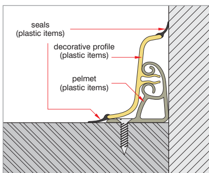
method of mounting splash-back batten in worktop colours, type I
