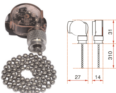
dielectric switch
