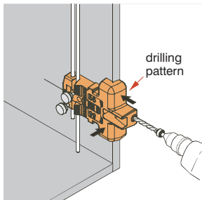
Drilling carcass under BLUMOTION insertion
