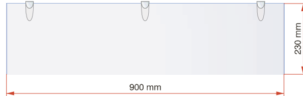
glass shelf "90"
