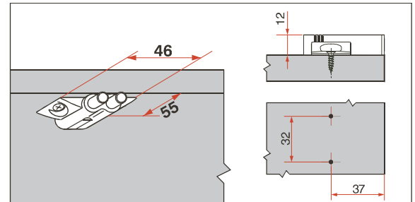
SPAX double plate mounting method
