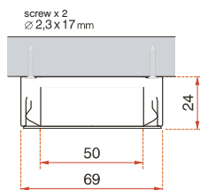
halogen 12V mounting, screwed, bulb type G4-20W
