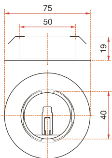
halogen 12V mounting, pressed, bulb type G4-20W
